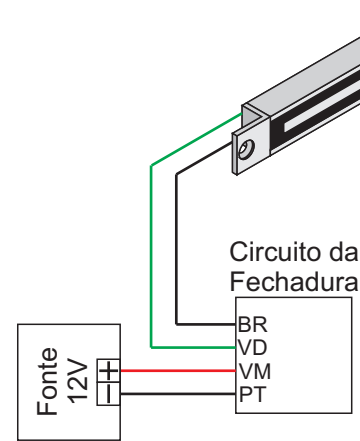
Clean 35 - 12V
