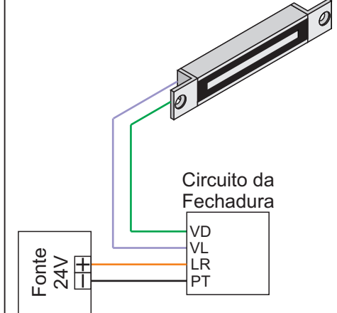
Clean 50 - 24V
