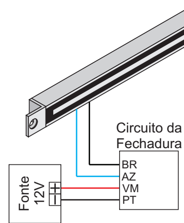
Clean 100 - 12V
