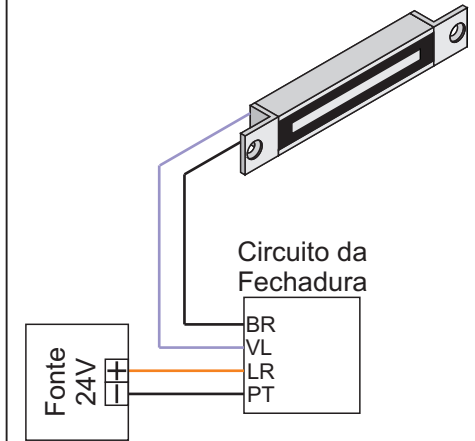
Clean 35 - 24V
